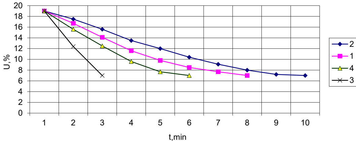
Fig. 2. Graph of the dependence of sunflower seed humidity on time for the height of the sunflower seed layer 15 mm (curve 1 and 3), 25 mm (curve 2 and 4), the distance from the IR emitter to the sunflower seed layer 40 mm (curve 1 and 2), 25 mm (curve 3 and 4) and for the heat flux density of the IR emitter of 5 \text{ kW/m}^2 .
