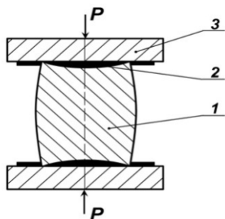
Figure 8. Scheme of deposition of a solid cylindrical sample with conditions of single axial compression: 1 – sample, 2 – foil, 3 – tool
