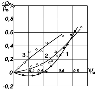
Figure 2. Dependence of plastic loosening of metals \Delta\rho/\rho_0 on the value of the plasticity resource used: \psi_u : •, o – compression; \Delta – torsion; x – stretch 1 – EI961 alloy; 2 – VT9 alloy; 3 – EP718 alloy
